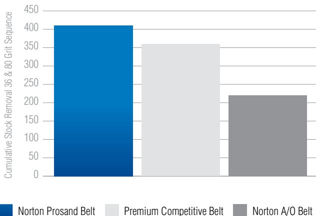
STOCK REMOVAL IN GRAMS OVER 6 MINUTES OF SANDING ON HARD MAPLE ON BELT SANDER
